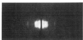
Fig. 5. A line-focus low-angle X-ray diffraction pattern of rat sciatic nerve in Krebs-Ringer's solution. The pattern was taken using 30 kV copper K\alpha nickel-filtered radiation, a specimen-to-film distance of 5.5 cm, an exposure time of 12 h and the radial period was d = 176 Å. The central region is over-exposed in order to show the higher orders of diffraction. Diffraction orders h = 3, 4, 5, 6, 8 , and 11 are clearly visible while weaker orders h = 7, 10 are just discernible.
