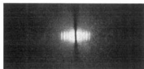
Fig. 3. A line-focus low-angle X-ray diffraction pattern of frog sciatic nerve in Ringer's solution. The pattern was taken using 30 kV copper K\alpha nickel-filtered radiation, a specimen-to-film distance of 5.5 cm, an exposure time of 12 h and the radial period was d = 171 Å. The central region is over-exposed in the reproduction in order to see the higher orders. Diffraction orders h = 2, 3, 4, 5, 6 and 11 are visible.
