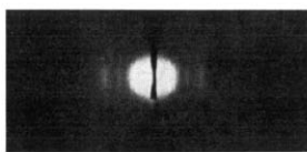
Fig. 3. A line-focus low-angle X-ray diffraction pattern of frog sciatic nerve in Ringer's solution. The pattern was taken using 30 kV copper K\alpha nickel-filtered radiation, a specimen-to-film distance of 5.5 cm, an exposure time of 12 h and the radial period was d = 171 Å. The central region is over-exposed in the reproduction in order to see the higher orders. Diffraction orders h = 2, 3, 4, 5, 6 and 11 are visible.
